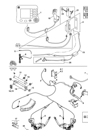
I.3, ETV-013088, AMATRON+, 1
